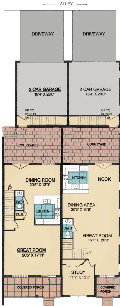
B A 1ST FLOOR PLAN
